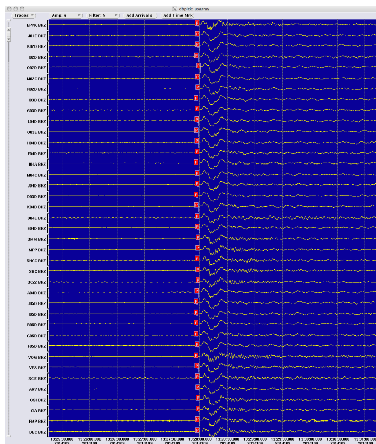
Screenshot from Vladik's computer of a magnitude 7.5 earthquake that occurred on April 19, 2014, in the Solomon Islands. The figure shows the waveforms across most or all of the Transportable Array stations, which are along the vertical axis; time is the x-axis.
