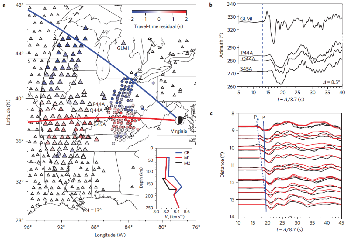
Figure 11. Summary of seismic observations of the Virginia earthquake (black beach ball) recorded by the Transportable Array stations (triangles). (a) Travel-time residuals (color triangles) and the ratio of long-period and short-period amplitudes multiplied by the travel-time residuals (colored circles at the midpoints) delineate an east–west corridor. (b) The recordings along the red profile are broad and late with deficient short-period energy, compared with those along the blue profile (e.g., Q44A versus GLMI). The model M1 (red lines in a.) predicts good waveform fits for the corridor (c). (c) The synthetics (red) show the interferences between P n , travelling in the upper lithosphere, and delayed P in the lower lithosphere. From Chu et al. [2013] .
